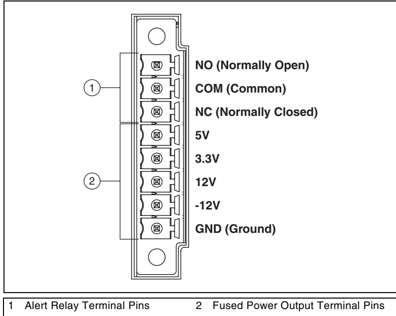
Figure 3-5. NI PXI-8250 Front Panel Connector Pinout Diagram
